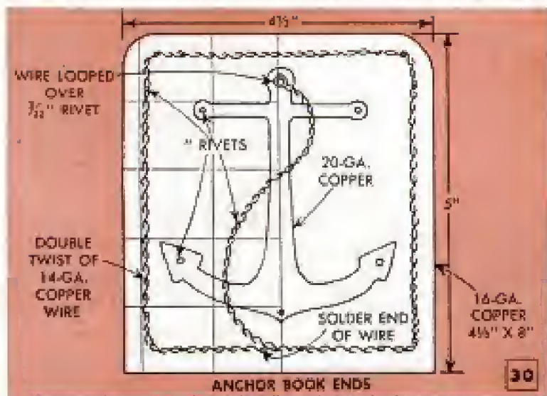
Photo above and detail and photo below show nautical book ends of riveted construction. Length of twisted wire provides "rope"
